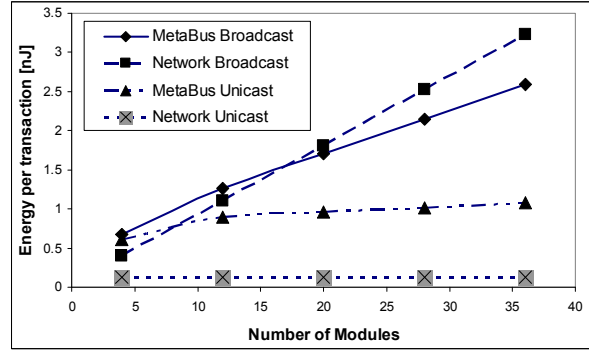
Figure 8. Bus and NoC unicast and broadcast energy per transaction.
