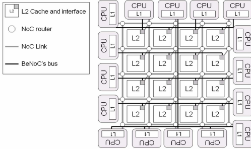
Figure 1. A BENOc-based CMP system, composed of 16 processors and 4x4 L2 caches.
